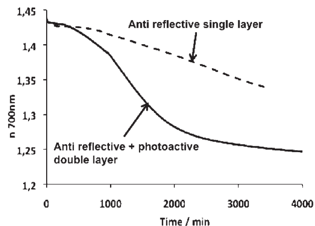
Figure 8. Evolution of refractive index with UV irradiation time for both single AR (AR2 sample) layer and AR-PA bilayer (AR2PA sample) systems contaminated with Lauric acid.
