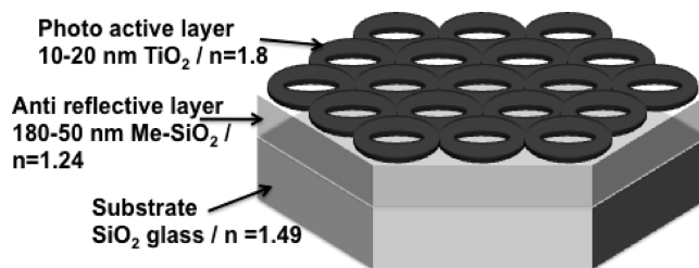
Figure 1. Scheme of the bilayer system composed of the thick AR underneath layer covered by the nanoporulated ultrathin PA layer.
