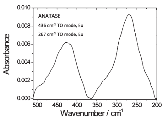
Figure 5. Far infrared absorption spectrum of a titania monolayer obtained on a AR2PA system.
