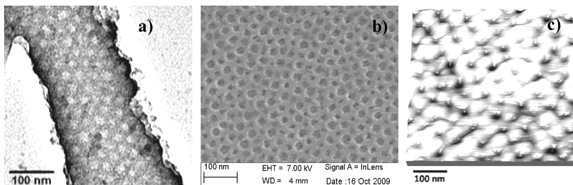
Figure 3. (a) TEM, (b) SEM, and (c) AFM images of the AR2PA bilayer system showing the presence of the 20 nm in diameter nanoporations at the surface.
